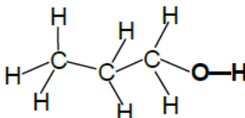
Compound E
